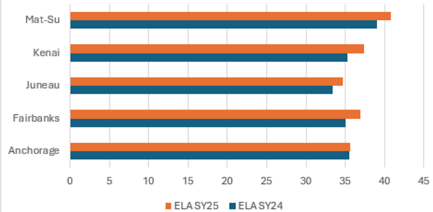
AK STAR ELA Score Comparison - SY24 to SY25
